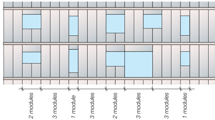
Good panel layout makes best use of 'module' size and location for all openings to reduce on-site panel cutting
